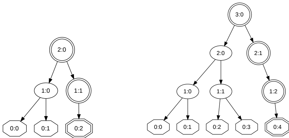
(a) Hashing 3 blocks: the tree has depth 3.
